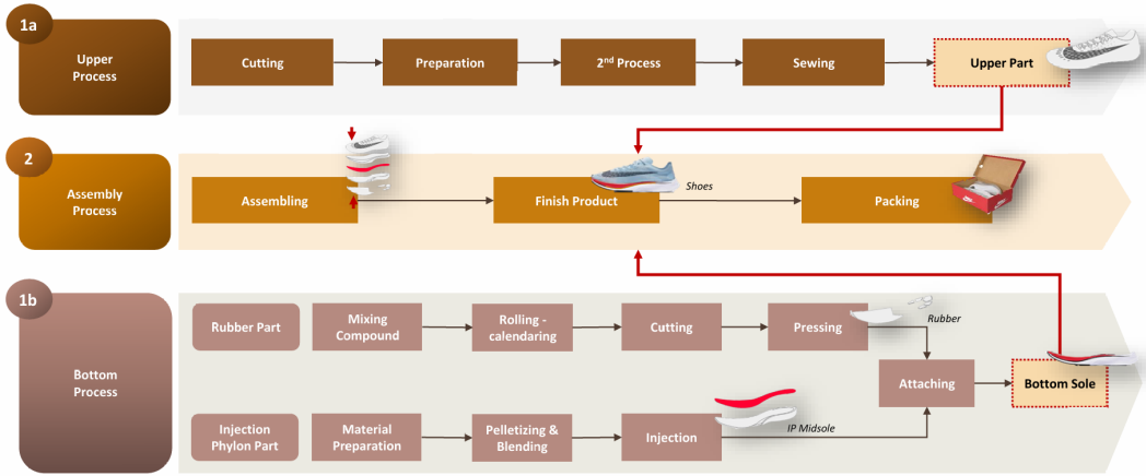
Figure 9. Factory production process for the footwear industry. Source: DEN (2025), based on site visits and interviews with footwear manufacturers.
