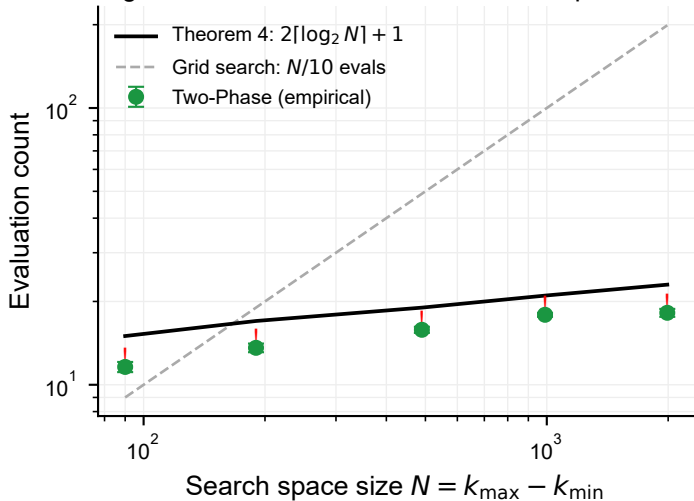
Figure 3: Evaluation Count vs. Search Space Size
