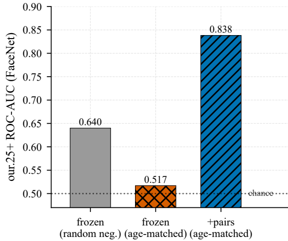
Fig. 1. The age shortcut: on an identity-only test (age-matched negatives), the frozen model falls to near-chance; fine-tuning on our pairs restores discrimination by identity.
