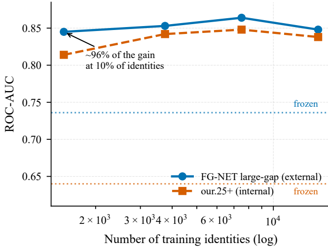
Fig. 2. Data-scaling law: external (FG-NET large-gap) and internal (our.25+) ROC-AUC vs. the number of training identities (log scale). Roughly 96% of the gain is reached at 10% of identities; dashed lines are the frozen baselines.
