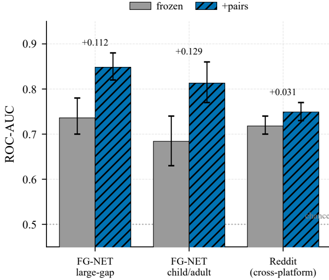
Fig. 6. External generalization. The +pairs gain over the frozen baseline (with 95% CIs) holds across three independent evaluations—FG-NET large-gap, a child↔adult FG-NET subset, and the cross-platform Reddit set—each well above chance. The gain is largest on the in-protocol FG-NET sets and smaller (but positive) on the noisier cross-platform Reddit set.
