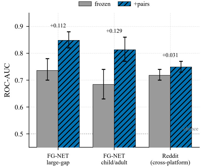
Fig. 2. External generalization. The +pairs gain over the frozen baseline (with 95% CIs) holds across three independent evaluations—FG-NET large-gap, a child \leftrightarrow adult FG-NET subset, and the cross-platform Reddit set—each well above chance. The gain is largest on the in-protocol FG-NET sets and smaller (but positive) on the noisier cross-platform Reddit set.
