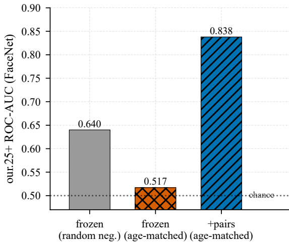
Fig. 3. The age shortcut: on an identity-only test (age-matched negatives), the frozen model falls to near-chance; fine-tuning on our pairs restores discrimination by identity.
