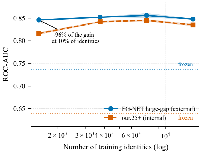
Fig. 2. Data-scaling law: external (FG-NET large-gap) and internal (our.25+) ROC-AUC vs. the number of training identities (log scale). Roughly 96% of the gain is reached at 10% of identities; shaded bands are \pm 1 std over three seeds and dashed lines are the frozen baselines.
