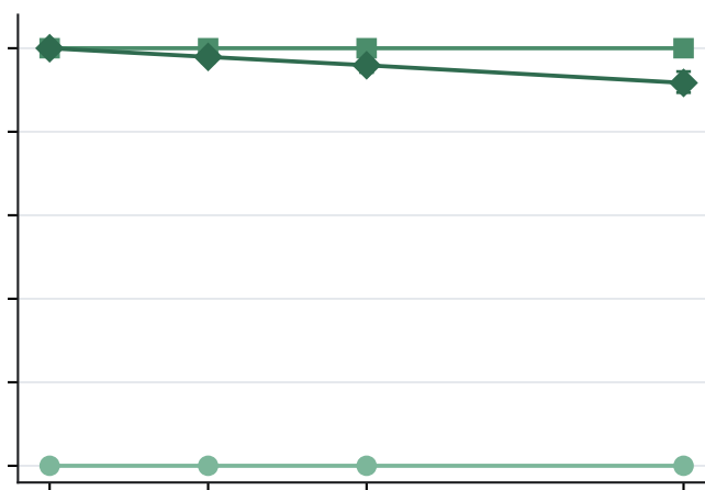
5 active candidates
