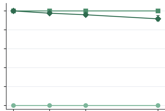
6 active candidates
