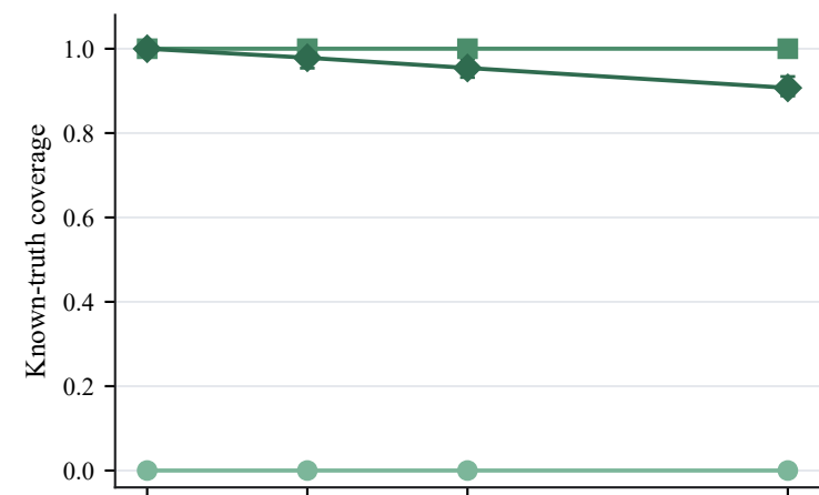
4 active candidates
