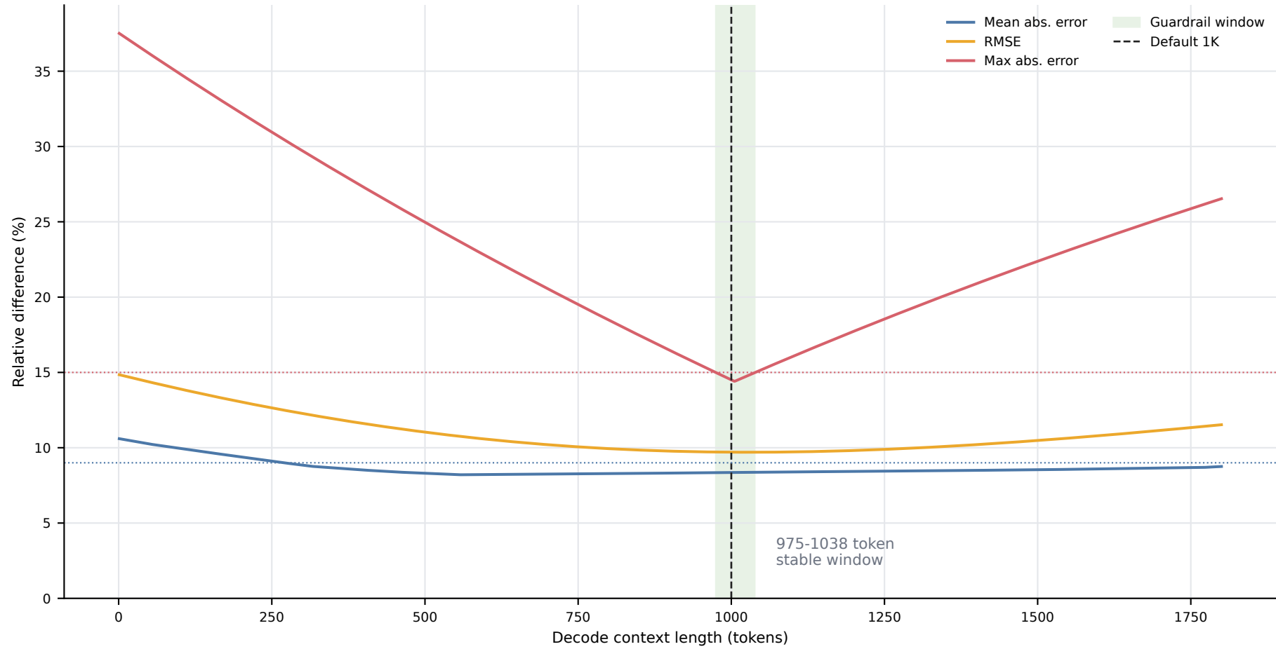
Inverse fit of public Figure 9 points supports a 1K context setting
