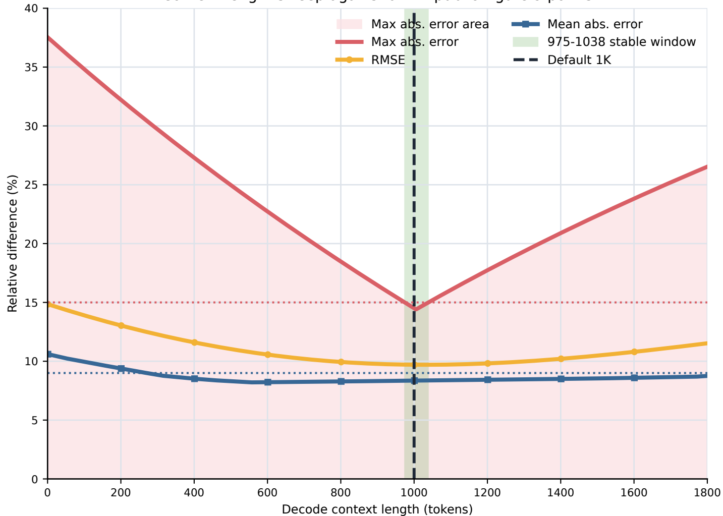
Context-length sweep against all 21 public Figure 9 points
