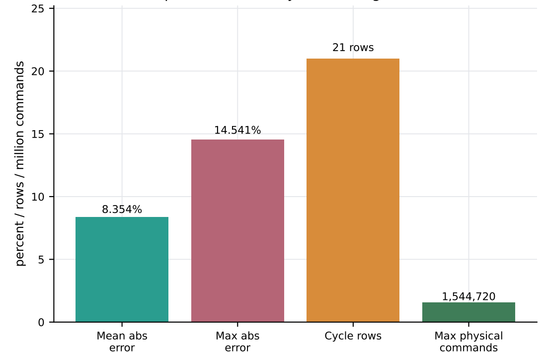
Reproduction and cycle-coverage checks
