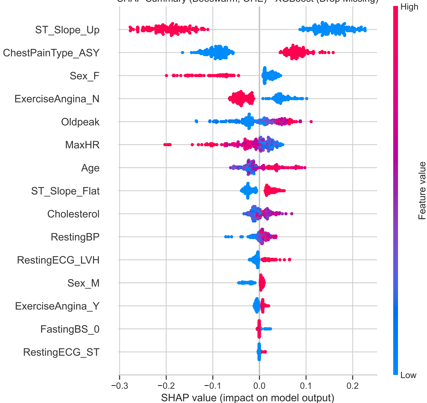
SHAP Summary (Beeswarm, OHE) - XGBoost (Drop Missing)
