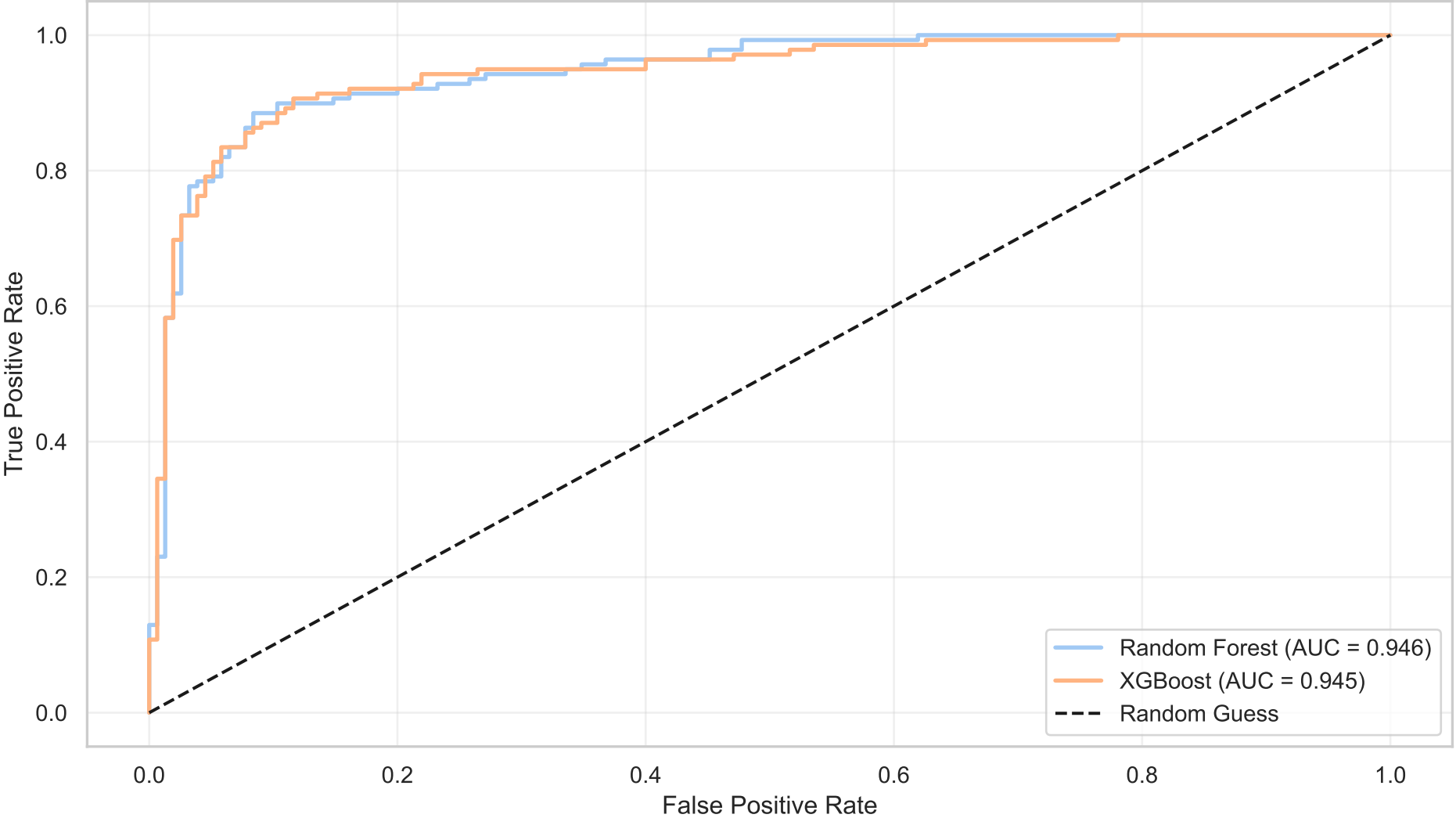
ROC Curve Comparison: RF vs XGB (Drop Missing)
