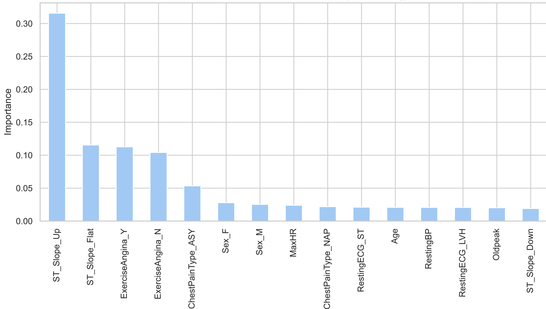
XGBoost - Top 15 Feature Importances (Drop Missing)
