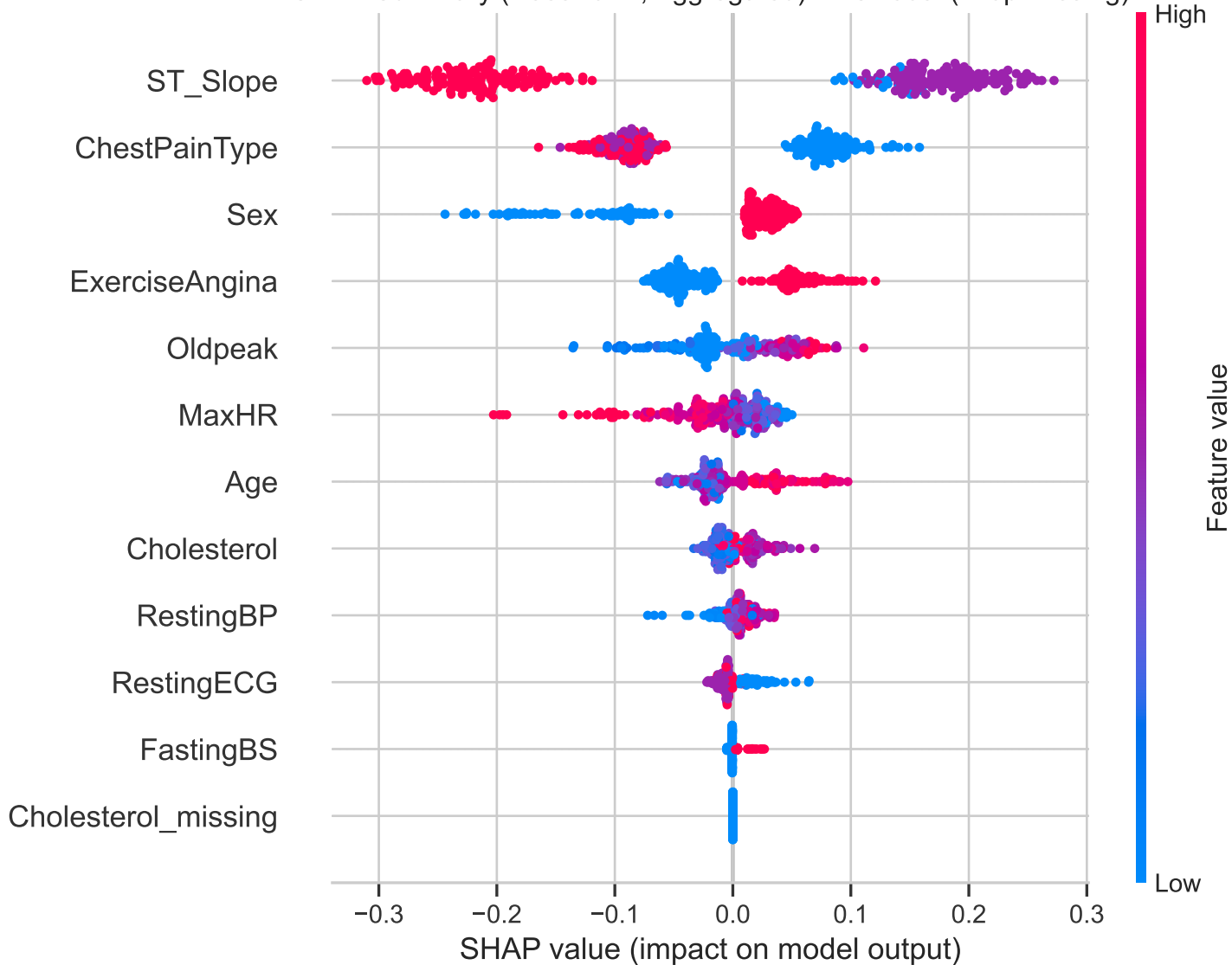
SHAP Summary (Beeswarm, Aggregated) - XGBoost (Drop Missing)
