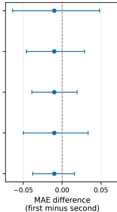
TurNuP - PMAK
