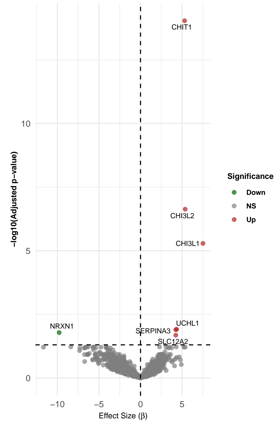
ALSvsHC (NONdel)
