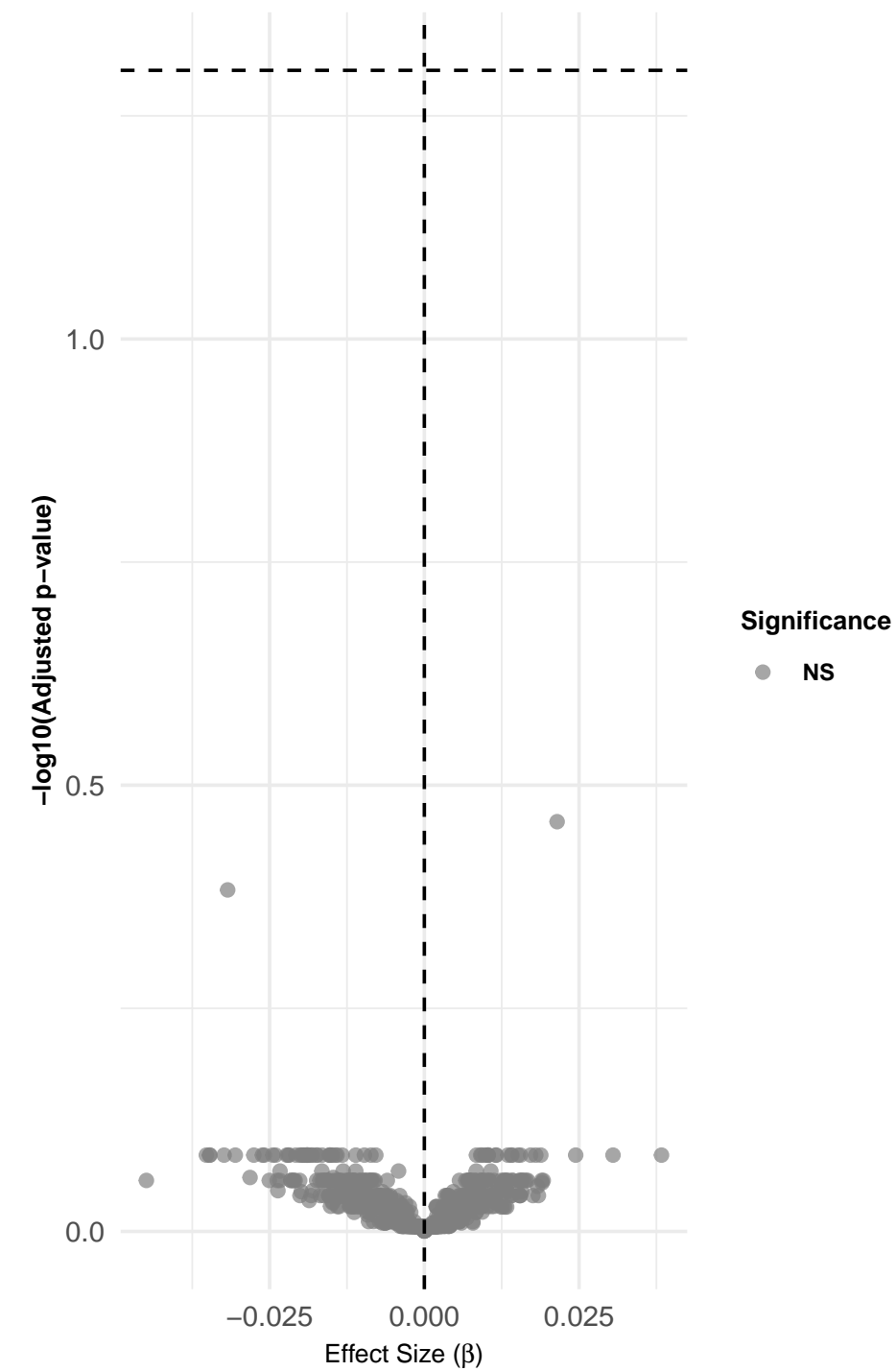
ECAS_SCORE (NONdel)
