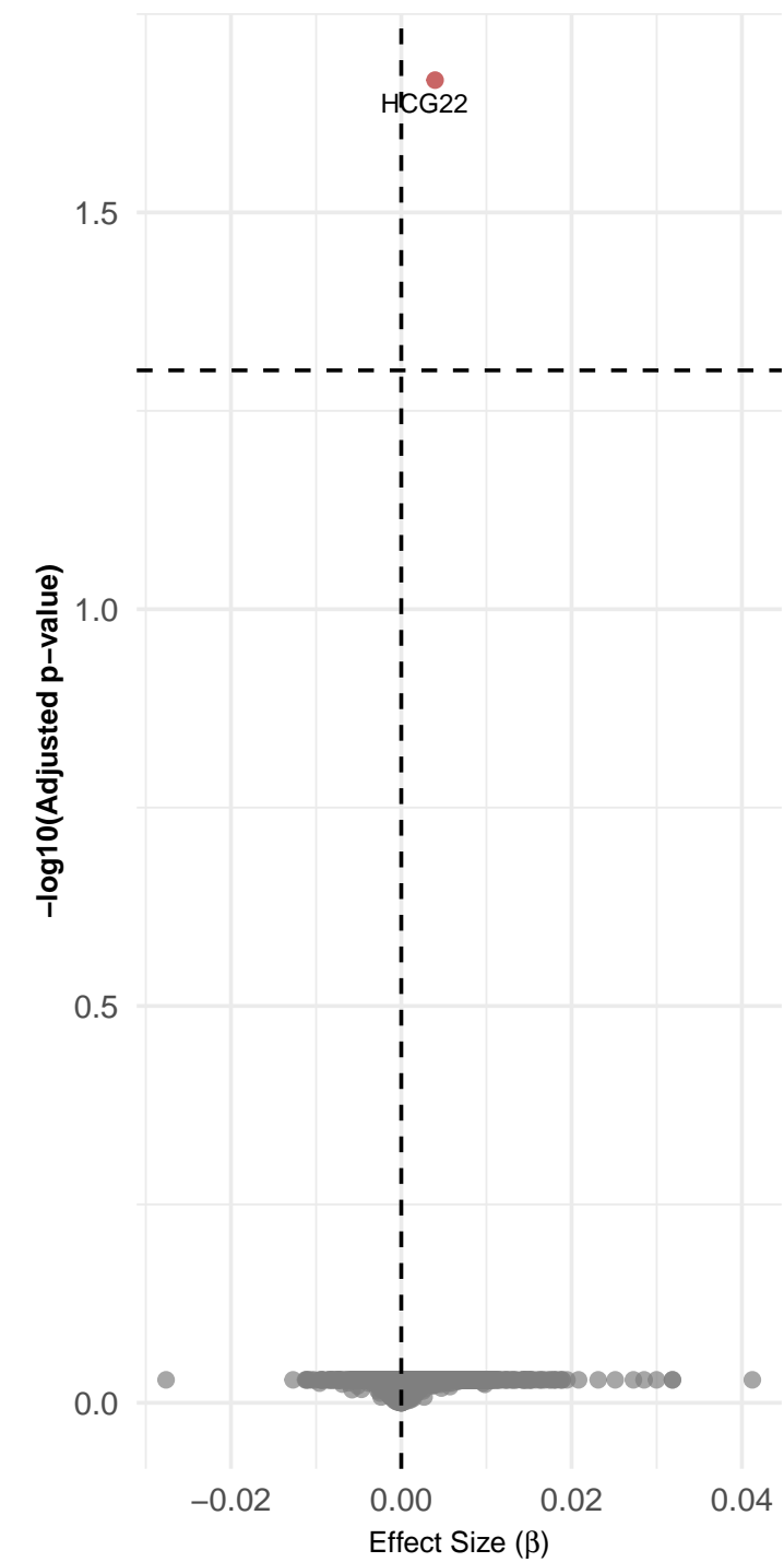
ECAS_SCORE (Olink)
