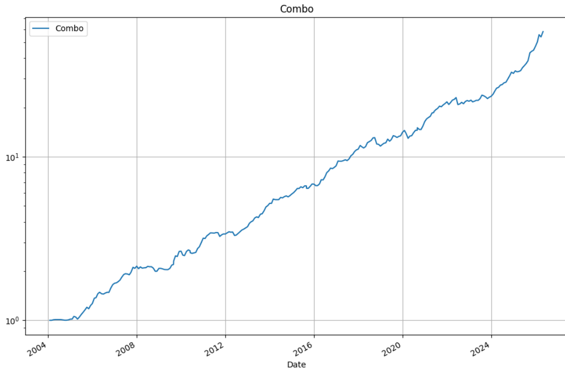
Figure 2: Combined portfolio equity curve with the strategic weights and the bond yield-curve filter, log scale.
