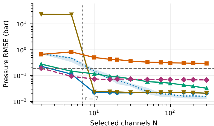
(c) P1, grid-wide channels
