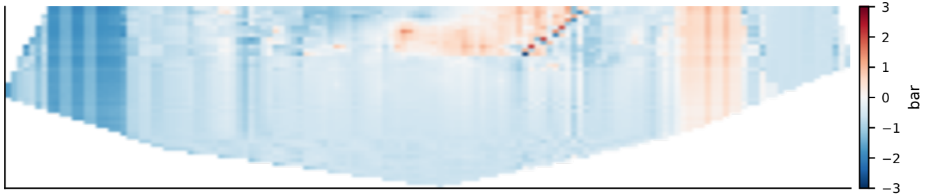
Error (estimate – reference): 10 DG wells, TBMD I1; RMSE = 0.735 bar
