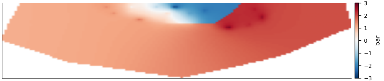
Error (estimate – reference): 10 DG wells, POD-E LS; RMSE = 0.140 bar
