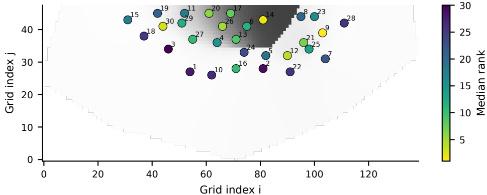
(E) Median conditioning-aware TBMD well rank
