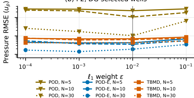
(b) P2, DG-selected wells
