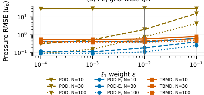
(a) P2, grid-wide QR
