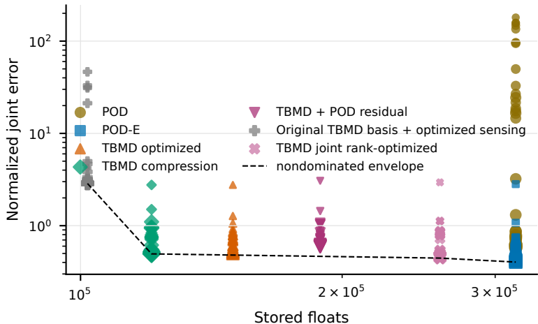
(G) Accuracy--storage--well-budget Pareto map
