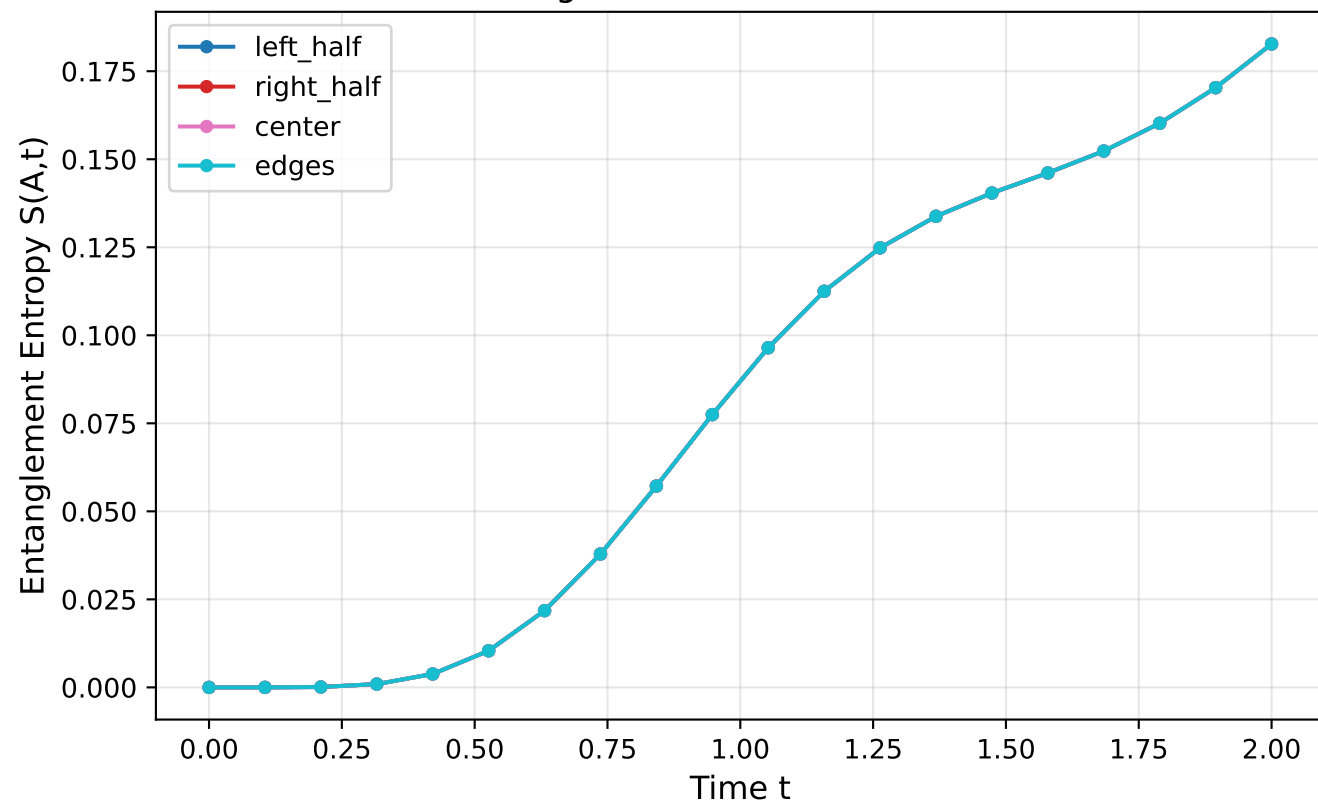
Linearity of Entanglement Growth
