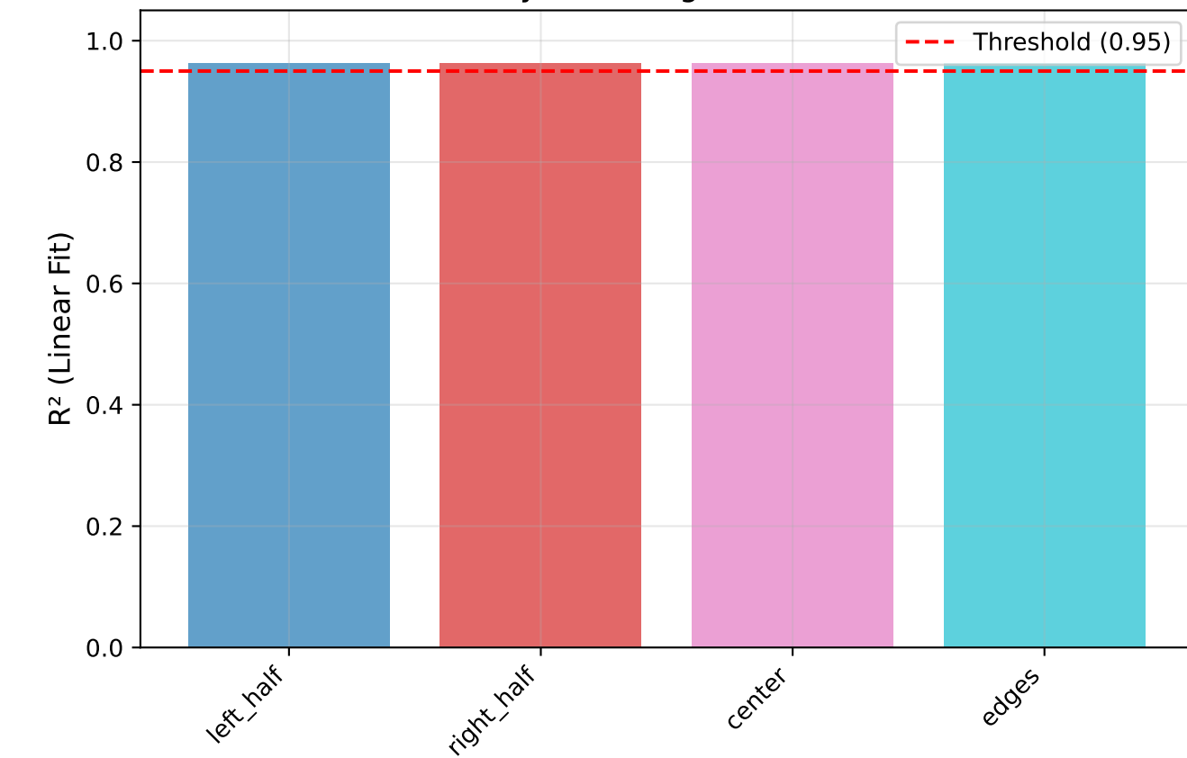
Linearity of Entanglement Growth
