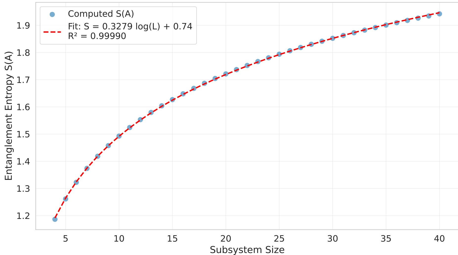
Area Law Verification
