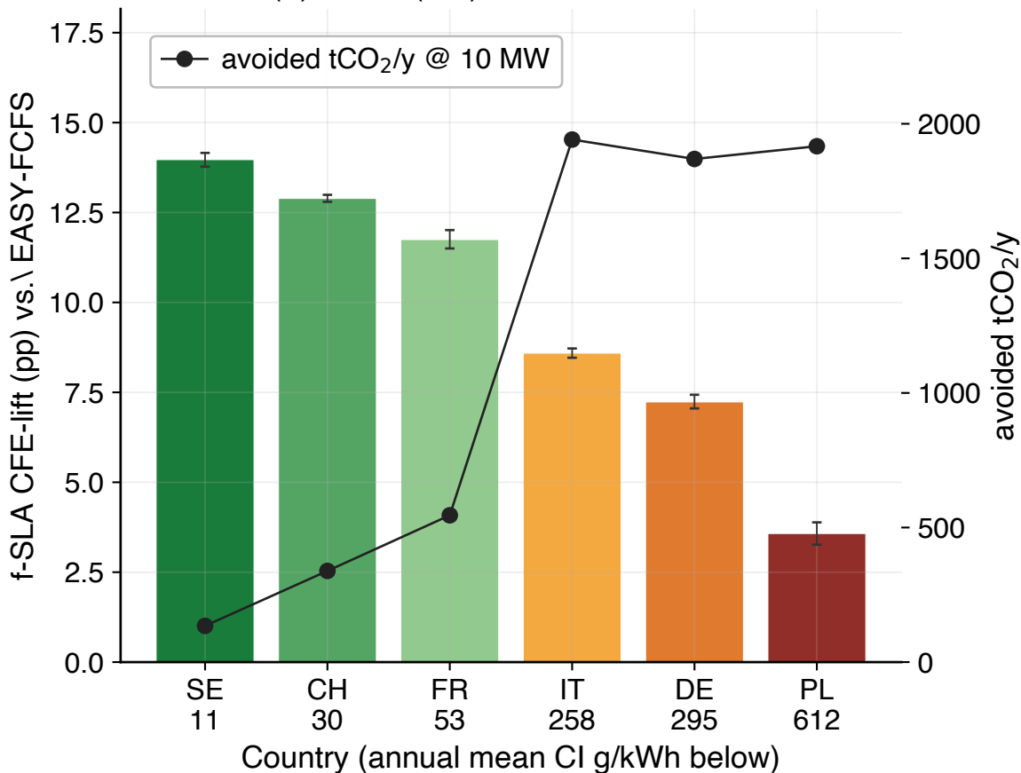
(a) f-SLA (M3) CFE-lift at 10 MW
