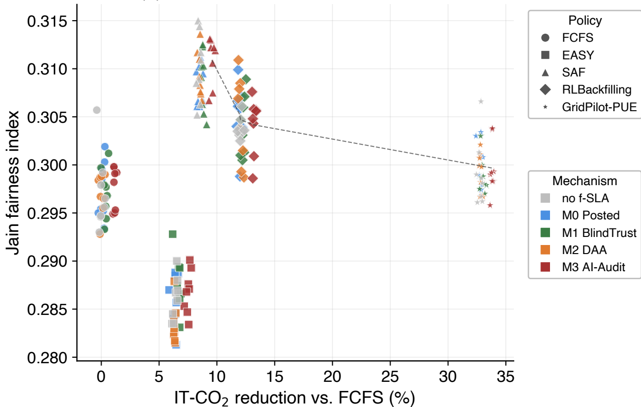
(a) Carbon vs. fairness Pareto scatter
