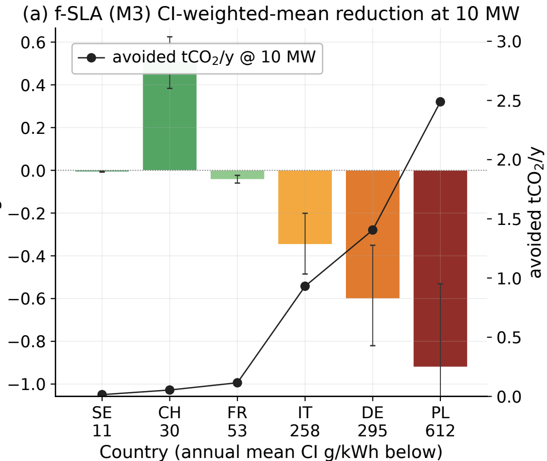
Effective CI reduction (g/kWh) vs. EASY-FCFS
