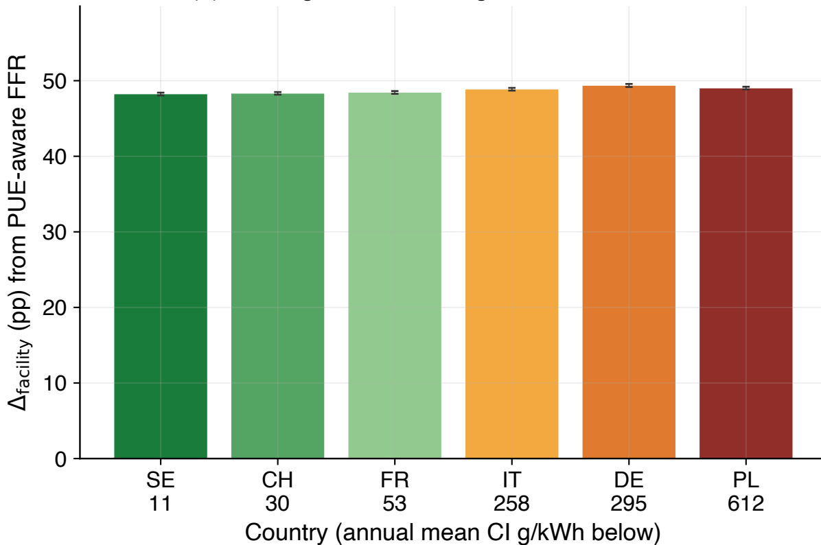
(a) Cooling-overhead drag closed at 10 MW IT
