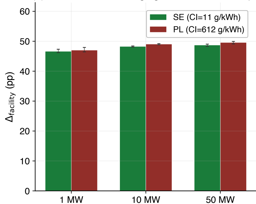
(b) Cluster-scale averaging shrinks the envelope
