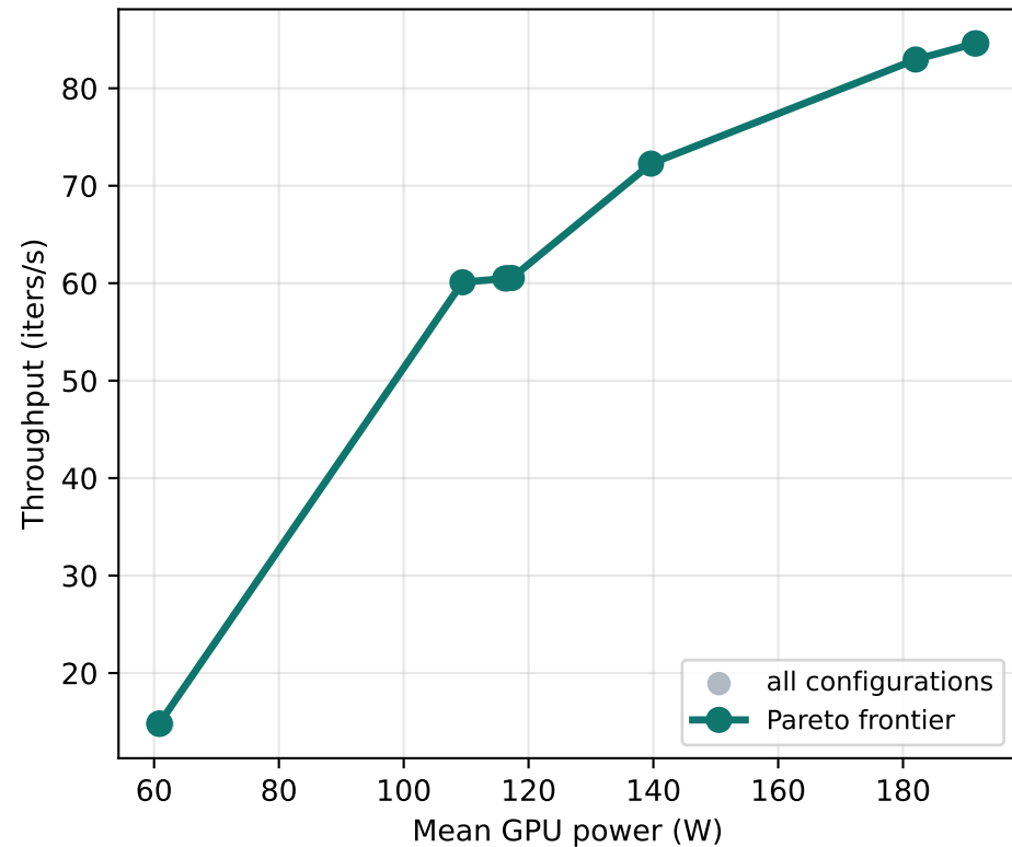
bursty_alternating
