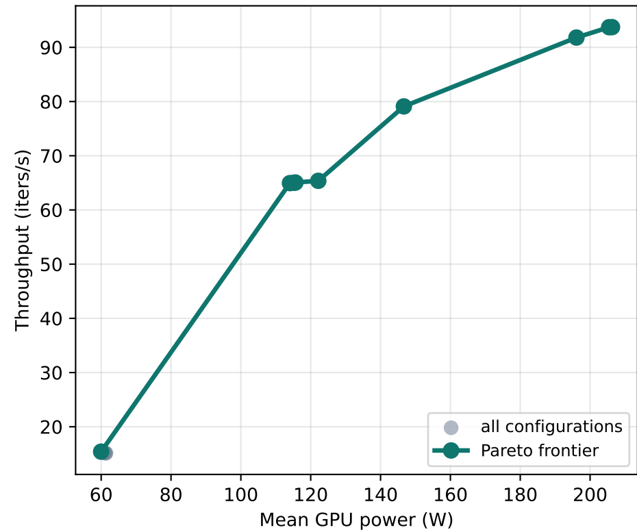
matmul_compute_bound
