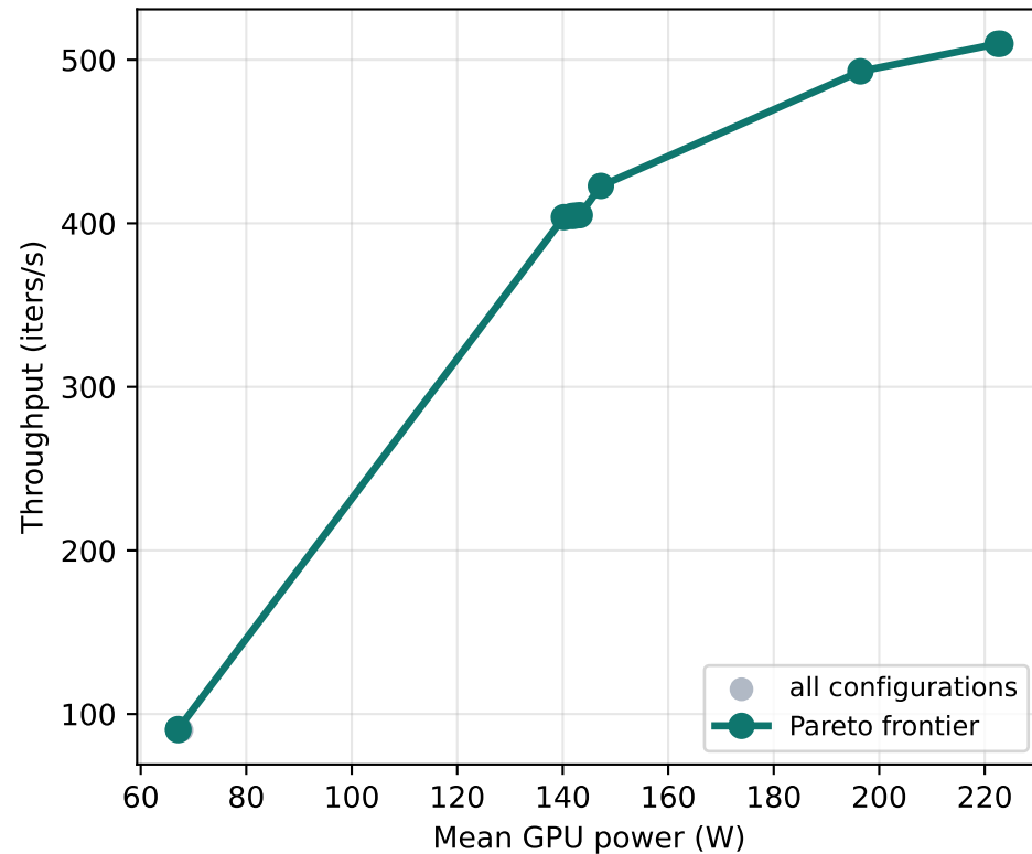
inference_memory_bound
