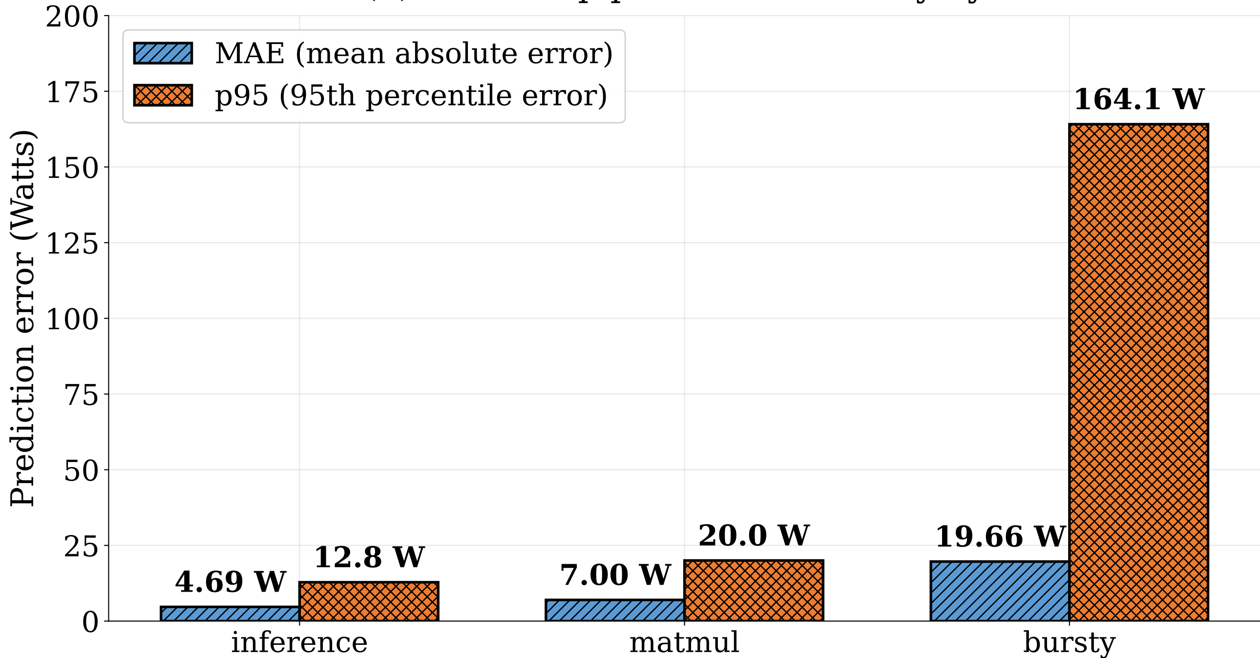
E3 — AR(4) outer-loop predictor accuracy by workload
