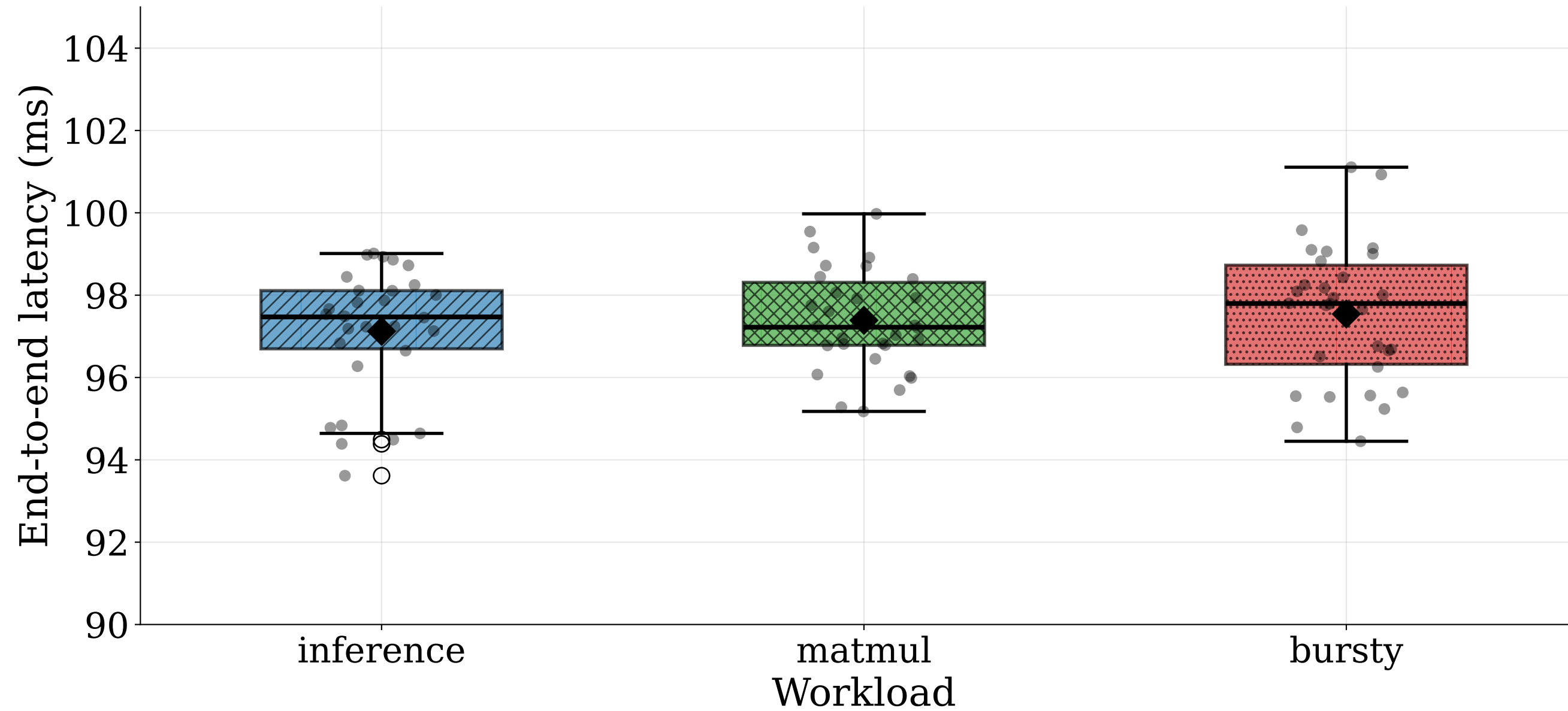
Per-trial latency distribution (90 trials, 30 per workload)
