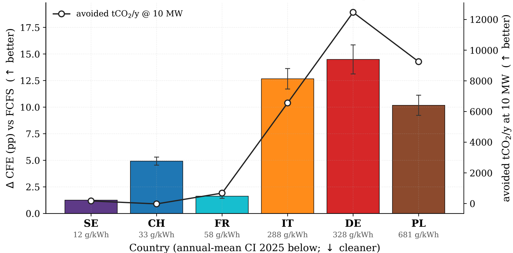
(a) f-SLA \Delta CFE at 10 MW — across the EU CI spectrum
