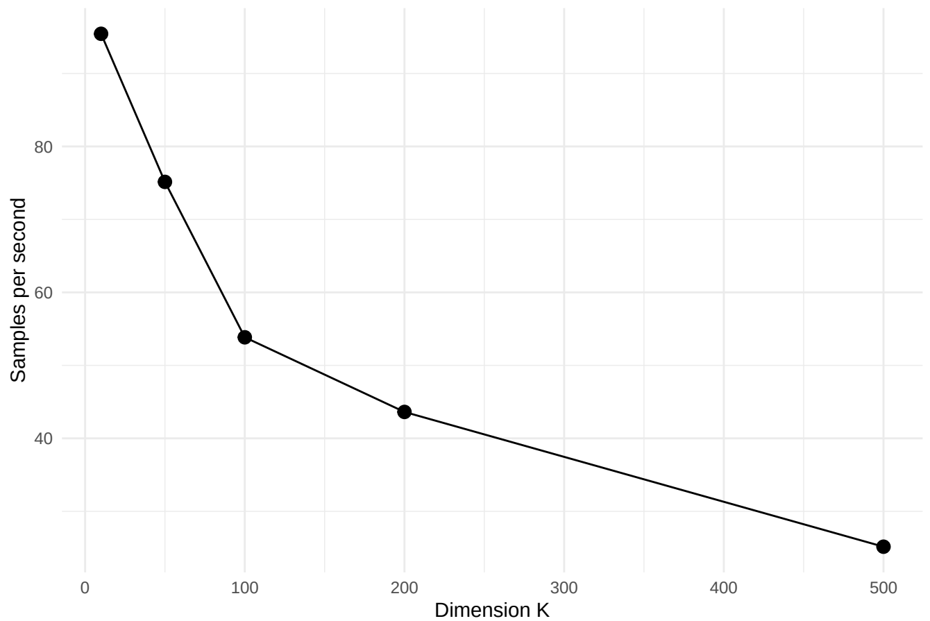
Sampling Throughput vs Dimension
