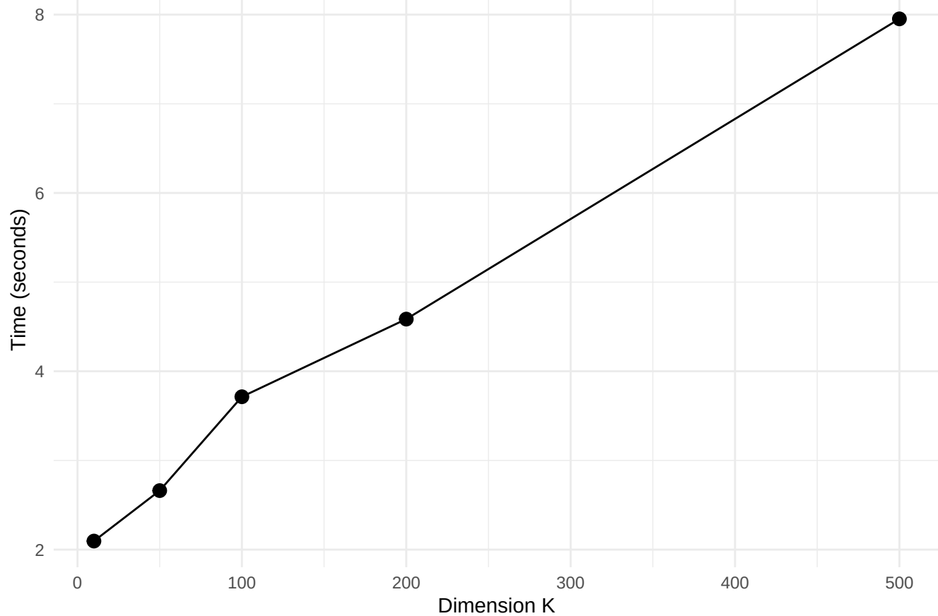
Computation Time vs Dimension
