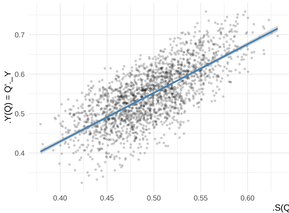
Correlated Effects (Good Surrogate)
