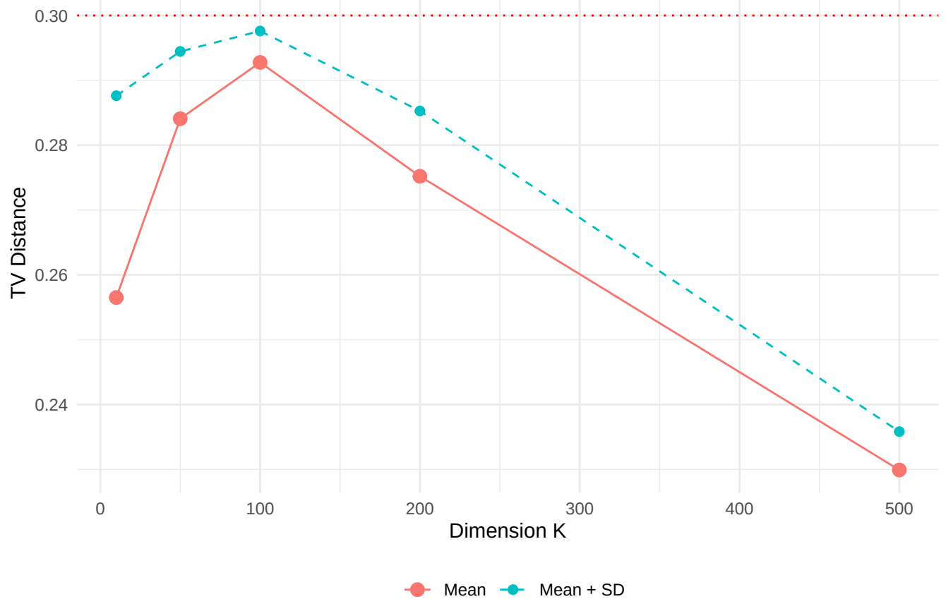
TV Distance Statistics vs Dimension
