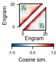
Example RS matrices (2% neurons)
