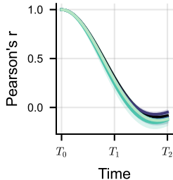
Population vector correlation
