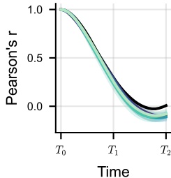
Tuning curve correlation
