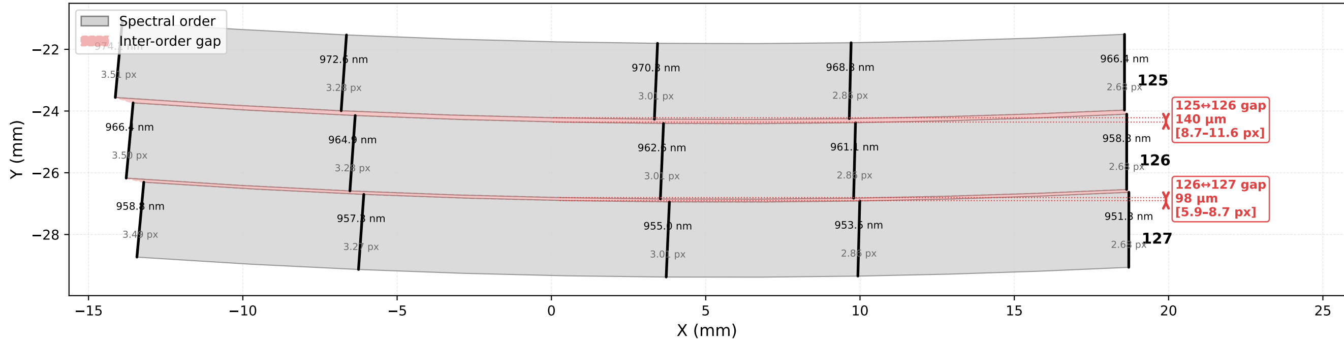
ANDES Y-band V36 — Orders 125-127 (inter-order gap)
