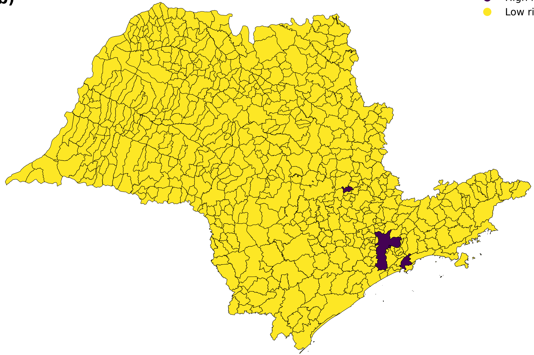
XGBoost
