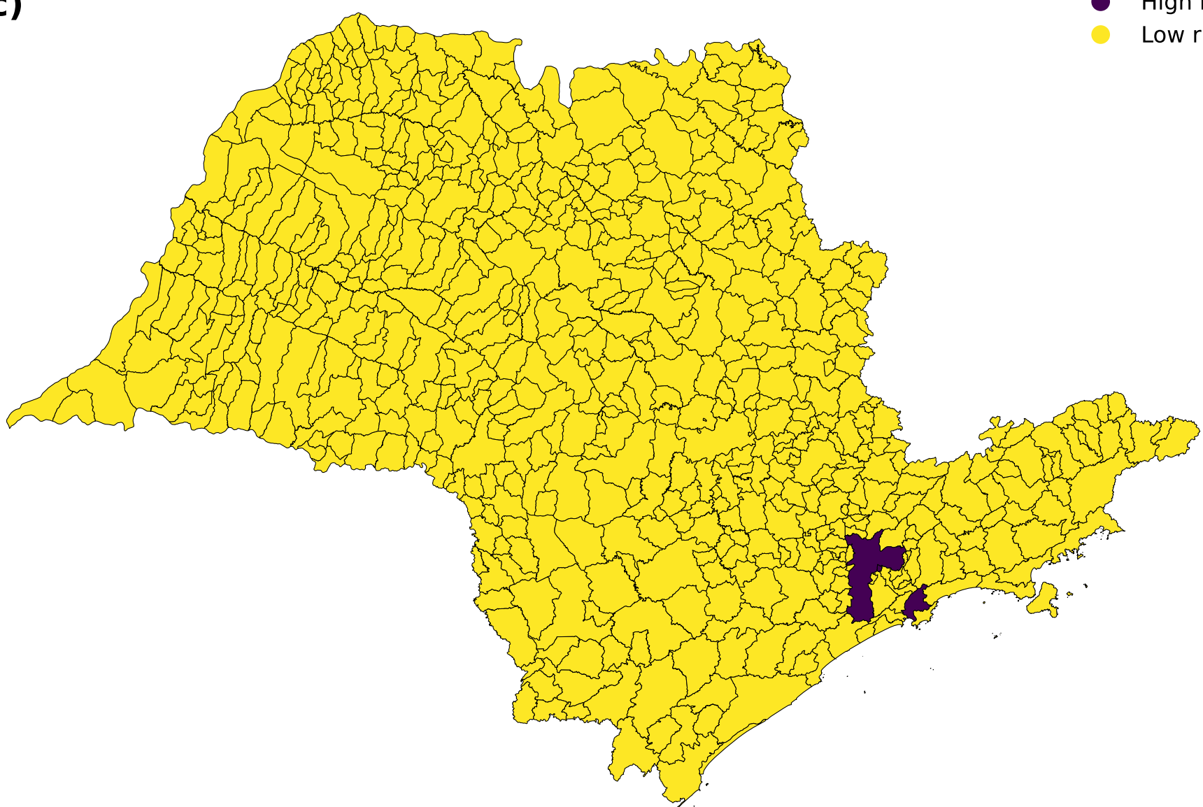
Random Forest
