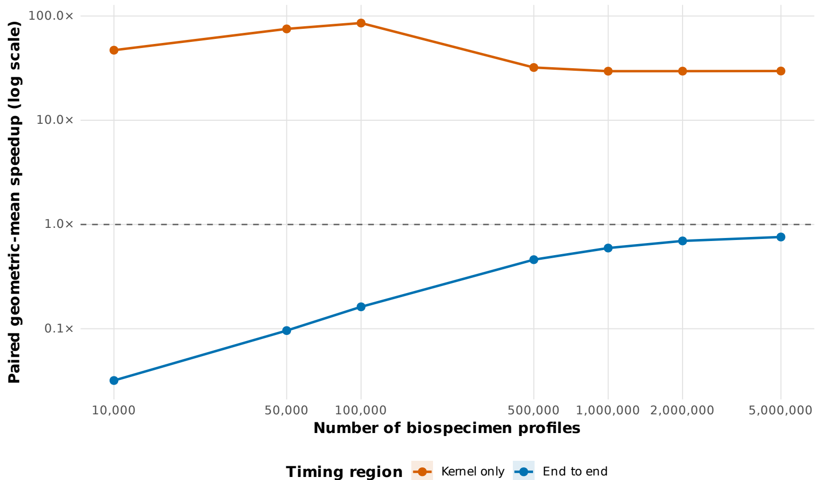
Figure S17. CUDA acceleration relative to C++ sequential
