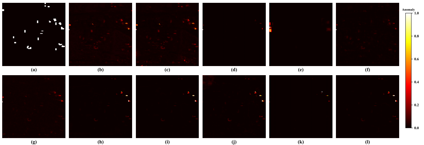
Fig. 8. HAD colored maps obtained by different algorithms for the El Segundo dataset. (a) Ground truth. (b) GRX. (c) FrFE. (d) LRX. (e) 2S-GLRT. (f) CRD. (g) LSDM-MoG. (h) GAED. (i) RGAE. (j) Auto-AD. (k) BS 3 LNet. (l) DirectNet.
