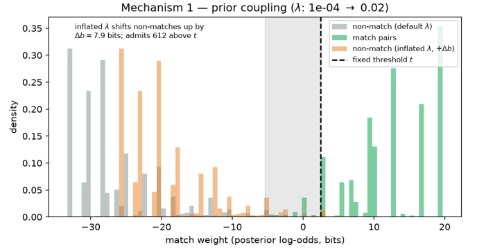
Fig. 1. Mechanism 1 (prior coupling) on NC-voter in posterior log-odds. The decision threshold is fixed at t = \log_2 \frac{\tau}{1-\tau} = 2.50 bits; the EM-estimated prior \lambda \approx 0.023 shifts the non-match distribution up by \Delta b \approx 7.9 bits (grey to orange), admitting about 612 non-match pairs in the shaded band as false positives. Prior coupling is secondary here to the Mechanism 2 recall collapse.
