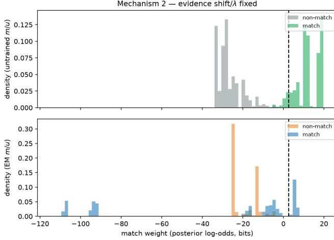
Fig. 2. Mechanism 2 (evidence shift) on NC-voter, \lambda fixed at 10^{-4} . Top panel: untrained m/u (match in green, non-match in grey); bottom panel: EM m/u (match in blue, non-match in orange). The EM-fitted weights move the match distribution sharply left (median 12.7 \rightarrow -8 bits) while the non-match distribution moves only slightly right (-28 \rightarrow -24), closing the separating gap; recall collapses as true matches are scored toward non-match territory. Dashed line: fixed threshold t .
