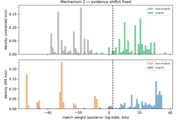
Fig. 4. Mechanism 2 on the synthetic duplicate-bearing benchmark (top: untrained m/u ; bottom: EM m/u ). The EM weights raise match weights (median 17 \rightarrow 24) and lower non-match weights (-25 \rightarrow -38), widening the gap rather than collapsing it, so Mechanism 2 is not the dominant failure on this data set.
