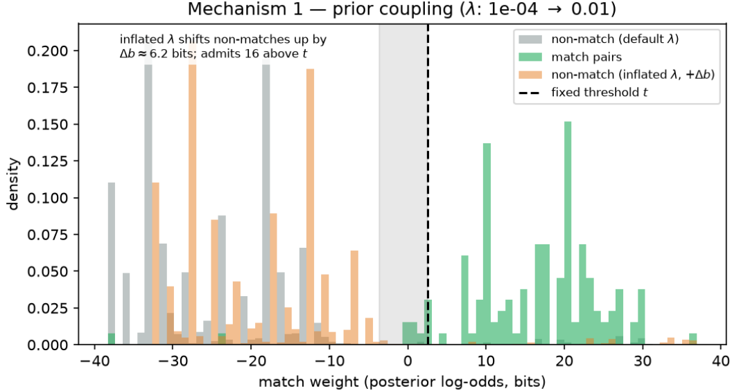
Figure 3: Mechanism 1 on the synthetic duplicate-bearing benchmark (posterior log-odds). Threshold fixed at t = 2.50 bits; EM’s fitted prior \lambda \approx 0.0071 shifts the non-match distribution up by \Delta b \approx 6.2 bits, admitting about 16 non-match pairs in the shaded band. (Artifact results/calibration/paradox_figures_synth_summary.json .)
