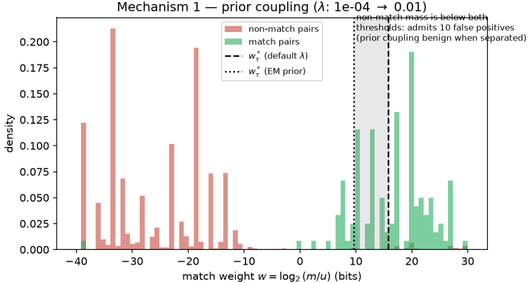
Figure 3: Mechanism 1 on the synthetic duplicate-bearing benchmark (fixed m/u ). Using EM’s fitted prior \lambda \approx 0.0069 shifts w_\tau^* from 15.8 to 9.7 bits; only about 10 non-matches lie in the shaded band.
