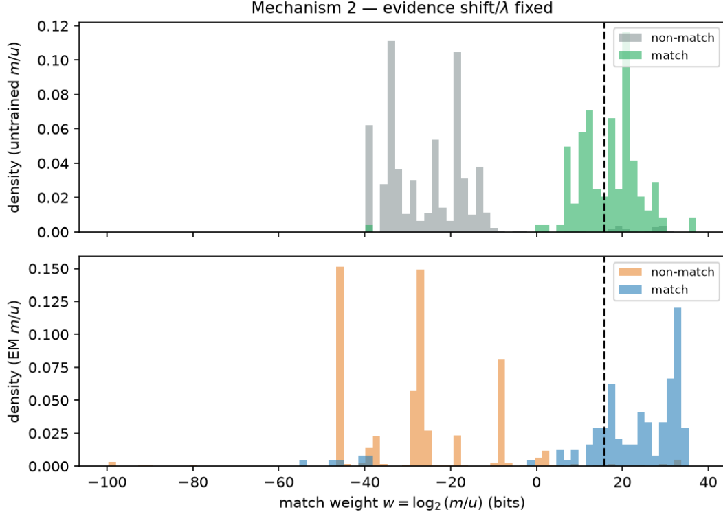
Figure 4: Mechanism 2 on the synthetic duplicate-bearing benchmark, \lambda fixed (top: untrained m/u ; bottom: EM m/u ). The EM weights raise match weights and lower non-match weights, widening the gap — so Mechanism 2 is not the dominant failure on this data set; prior coupling is.
