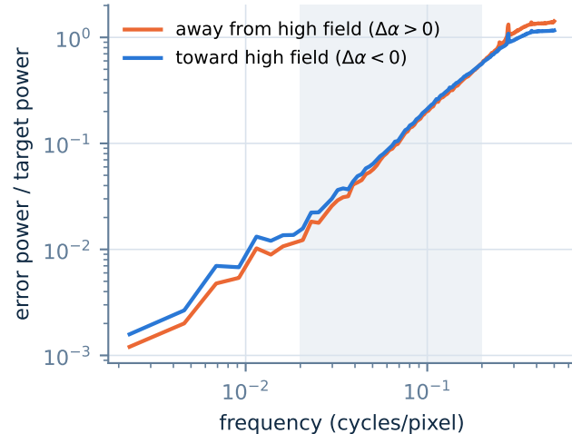
c · relative error, by direction
