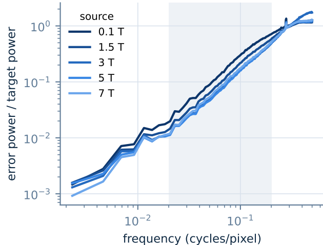
a · relative error, by source field
