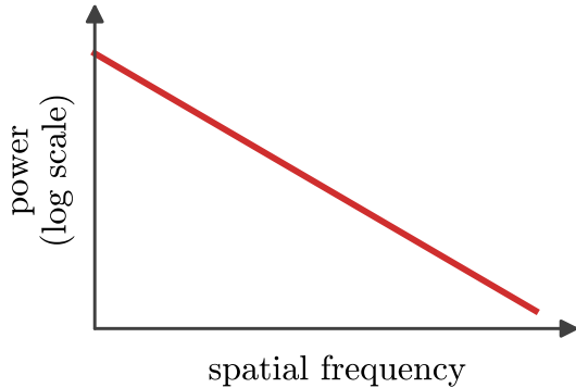
natural image
