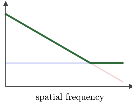
noisy image
