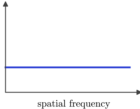
Gaussian noise
