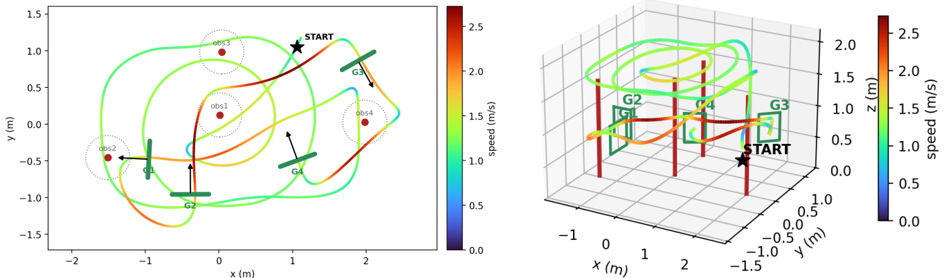
Fig. 5. A run on the fixed competition track ( final.toml ), from the simulator, colored by speed. Left, top-down: the wide loops are the blind spiral search that covers the arena; once all four gates are found the drone races them, slow (blue to green) at the gates and tight turns and fast (orange to red) on the straights. Green bars are the gate openings with the crossing direction, red marks are obstacles with their keep-out and the star is the start. Right, three-dimensional: the search spiral runs high, above the obstacle poles, then the drone descends to race the gates.
