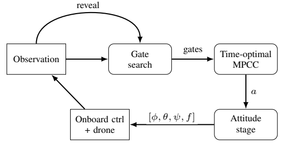
Fig. 1. Controller structure after takeoff. The drone reads the observation, the search discovers the gates, a time-optimal MPCC races them and the attitude stage produces the command. A gate is revealed when the drone passes within 0.7 m of it.
