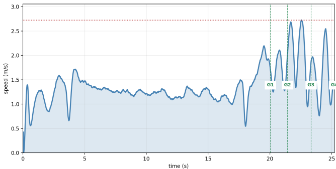
Fig. 6. Speed against time on the fixed competition track. The long low-speed section is the blind spiral search covering the arena, and the short high-speed section is the race through the four discovered gates. The search, not the racing, sets the lap time.
