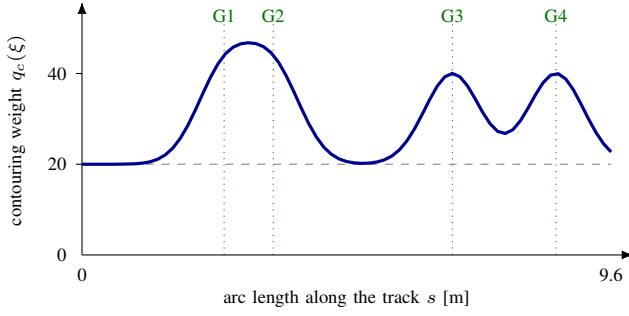
Fig. 4. The gate-aware contouring weight along the track, computed from (9) for the competition layout. The weight sits at a low base on the straights and rises to a peak at each gate (G1 to G4), so tracking is stiff only where a gate must be threaded. Gates whose arc positions fall within the window merge into a single wider peak.
