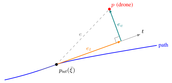
Fig. 4. Contouring geometry. At the reference point p_{\text{ref}}(\bar{\xi}) the path has tangent t . The error from the drone position p splits into a lag part e_l along t and a contouring part e_c across it, and the two meet at a right angle at the foot. Together they form the full error e . MPCC penalizes the contouring error hard and the lag softly, and rewards progress so the drone flies as fast as the constraints allow.
