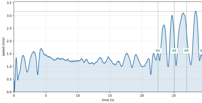
Fig. 7. Speed against time on a final.toml draw. The long low-speed section is the blind spiral search covering the arena, and the short high-speed section is the race through the four discovered gates. The search, not the racing, sets the lap time.
