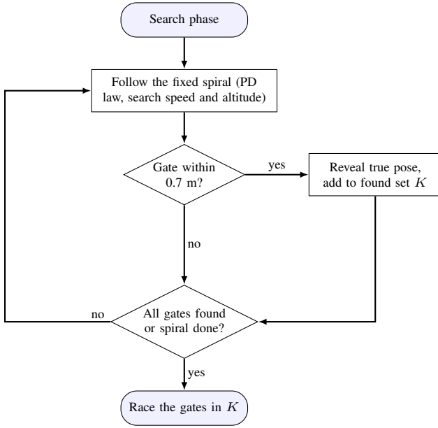
Fig. 3. Gate search, run once per control tick in the search phase. The drone follows the fixed spiral and reveals any gate that comes within 0.7 m in the horizontal plane, adding it to the found set K . It keeps sweeping until every gate is found or the spiral ends, then hands K to the racing stage.
